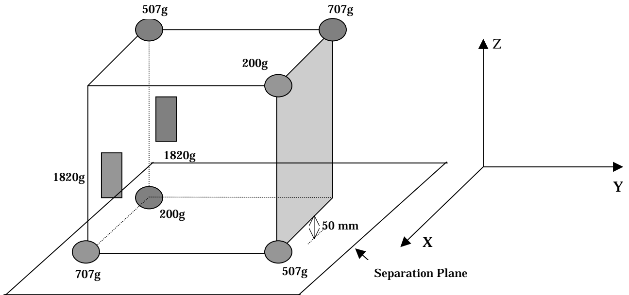
Figure.1: Mass and Allocation of BW(Balance Weight)
